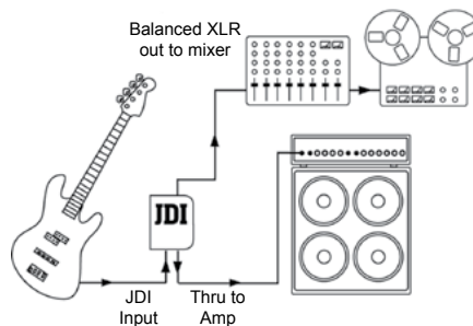
Fig. A: JDI used with on-stage instrument amplifier.
